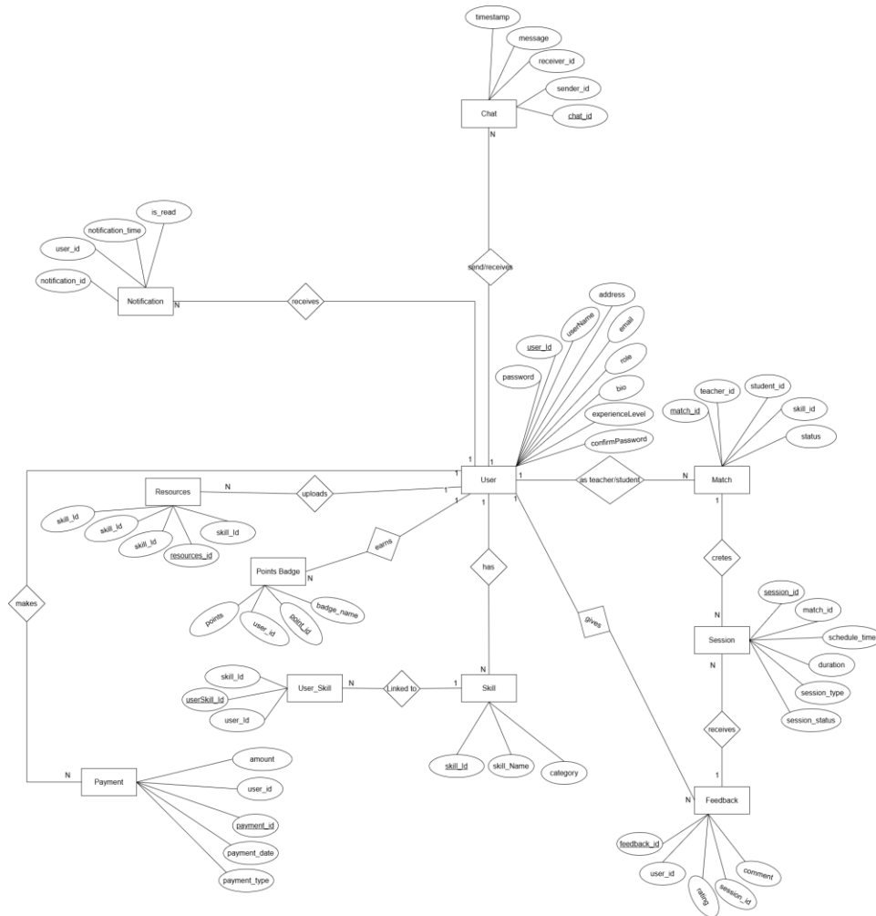
Figure 1: ERD
